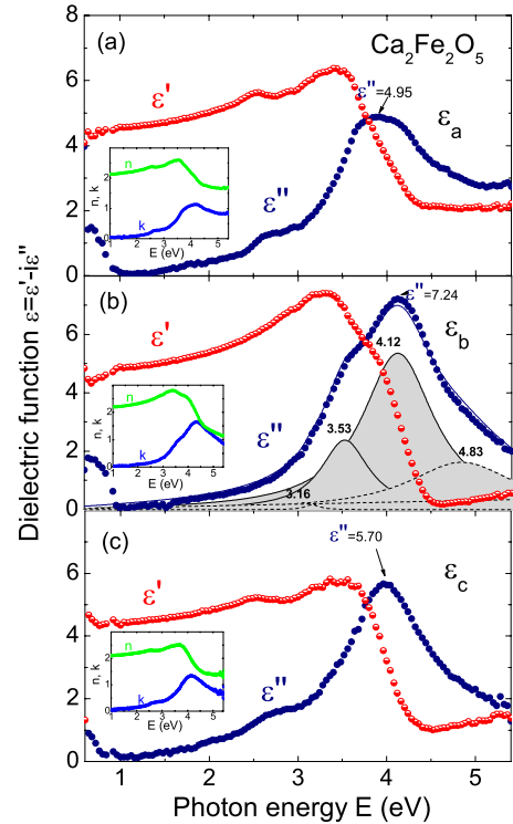
FIG. 8. (Color online) The dielectric function spectra in calcium ferrite \text{Ca}_2\text{Fe}_2\text{O}_5 for three main polarizations. Insets show indices of absorption and refraction.
