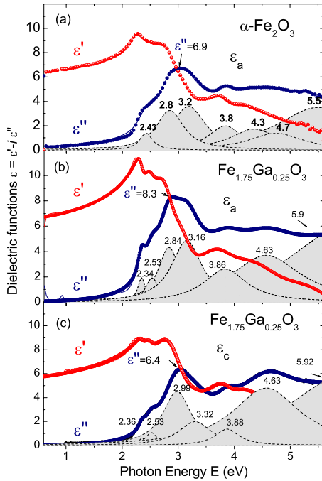
FIG. 5. (Color online) The dielectric function spectra of hematite \alpha\text{-Fe}_2\text{O}_3 (a) and gallium-substituted hematite \alpha\text{-Fe}_{2-x}\text{Ga}_x\text{O}_3 with [(b) and (c)] x=0.25 .
